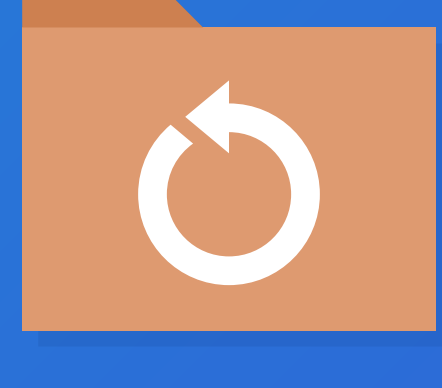
Restoring backups
